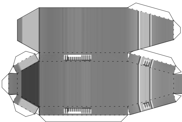
conning tower (middle & top)
